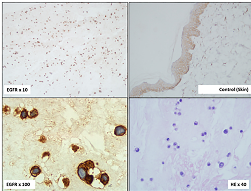
FIG. 4. Immunocytochemical staining for EGFR expression level of UPCI-SCC-131 cell was performed using EGFR mouse monoclonal antibody (1 : 15 dilution) with Leica Bond Autostainer. EGFR-immunostained areas were shown at a magnification of 100x. The UPCI-SCC-131 cell showed strong EGFR staining intensity. EGFR, Epidermal Growth Factor Receptor.
