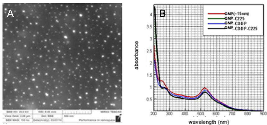
FIG. 2. A-B. The characterization of GNP was carried out using scanning electron microscope (SEM) and UV-visible spectroscopy. (A) SEM image showed that approximately 15 nm in diameter and spherical GNPs. (B) UV-vis spectrum of GNPs with CDDP and/or CTX showed absorption spectra at different wavelengths.
