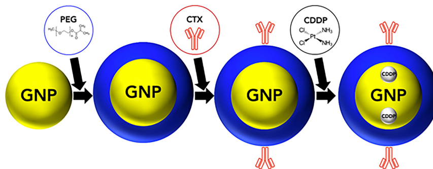
FIG. 1. A schematic illustration of the development of PEG-functionalized and CDDP- and CTX-loaded nanodrug complex. GNPs were reduced using sodium citrate, mixed with PEG, and incubated with CTX and CDDP to synthesize nanodrug complex. GNP, Gold nanoparticle; PEG, Polyethylene Glycol; CDDP, cisplatin; CTX, Cetuximab.
