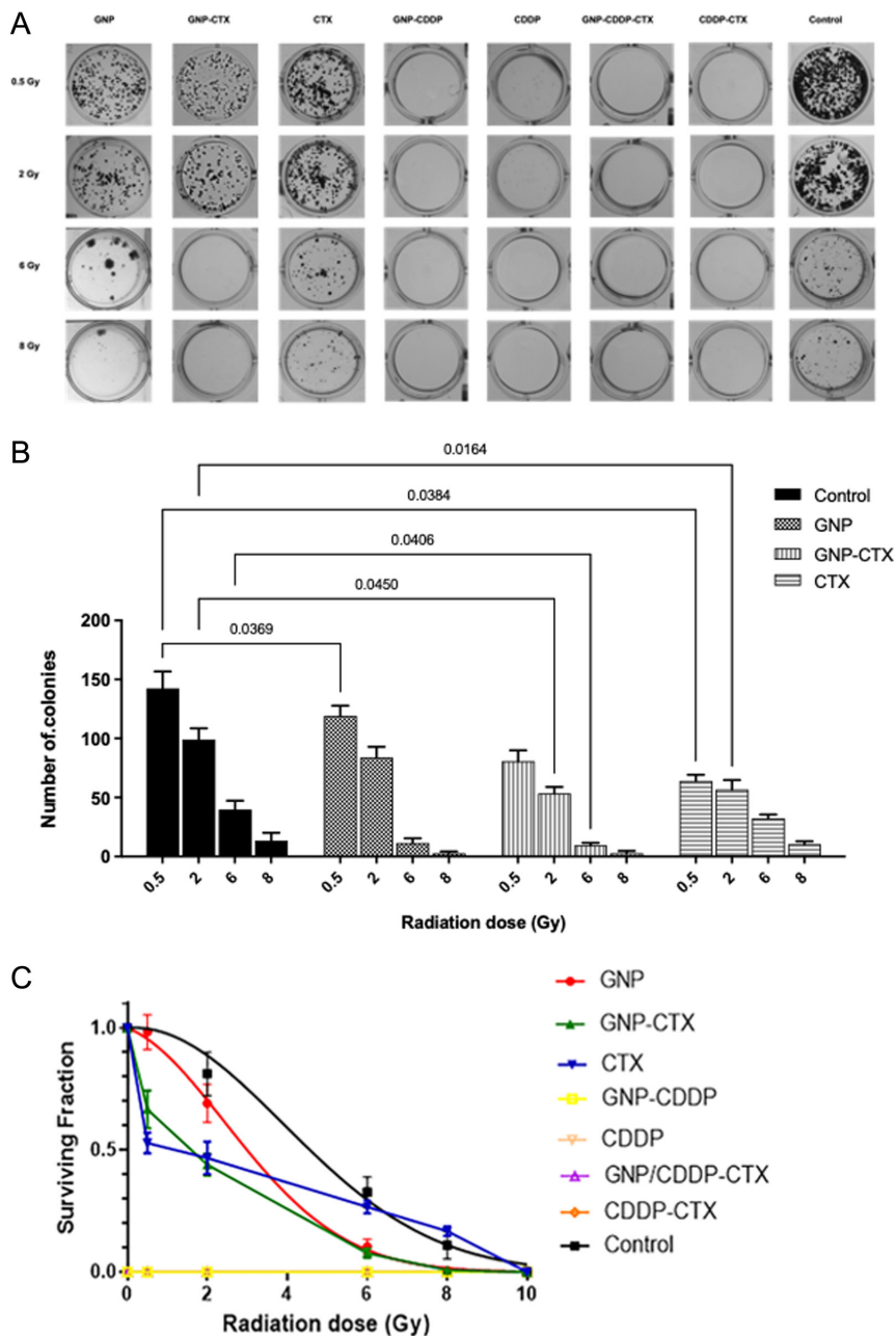
FIG. 7. A-C. Radiosensitization effects of GNPs in UPCI-SCC-131 cells (A) Images of colonies containing functionalized GNPs exposed to irradiation at different megavoltages was determined using clonogenic survival assay (B) Numbers of colonies was decreased with increasing doses of radiotherapy (C) The effects of GNPs on UPCI-SCC-131 cell survival was calculated by surviving fractions (SF), which showed the actual efficacy of the radiation effect on the cells. Data are expressed as mean ±SD (n = 3). GNP, Gold nanoparticle; CDDP, Cisplatin; CTX, Cetuximab.
