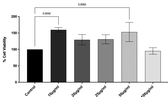
FIG. 5. The percentage of cell viability in different concentrations (10, 20, 25, 50, and 100 µg/mL) of 15 nm GNP-treated UPCI-SCC-131 cells for 48 hours. Data are expressed as mean ± SD ( n = 3). * P ≤ .05. GNP: Gold Nanoparticle.
