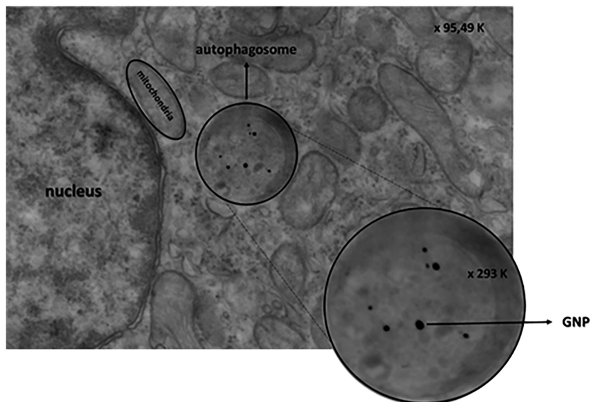
FIG. 3. Transmission electron microscopy images of UPCI-SCC-131 cells after exposure to 15 nm GNPs for 48 hours. The aggregates of GNPs were located in autophagosomes throughout the cell ( \times 95\text{ K} and \times 293\text{ K} ). GNP, Gold nanoparticle.
