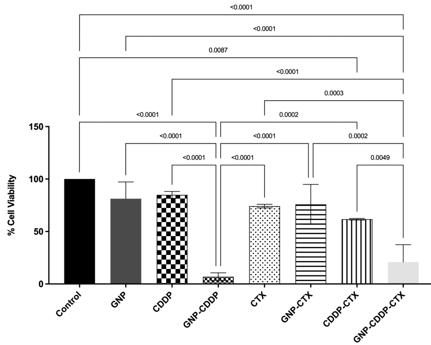
Supplementary FIG. 1. Cell viabilities of NIH-3T3 cells studied by using the x-CELLigence RTCA system, and the cells were treated in medium containing 25 \mu\text{g}/\text{mL} GNPs, 2.5 \mu\text{g}/\text{mL} CDDP, and 25 \mu\text{g}/\text{mL} CTX. Data are expressed as mean \pm SD ( n = 3 ). * P \leq .05
