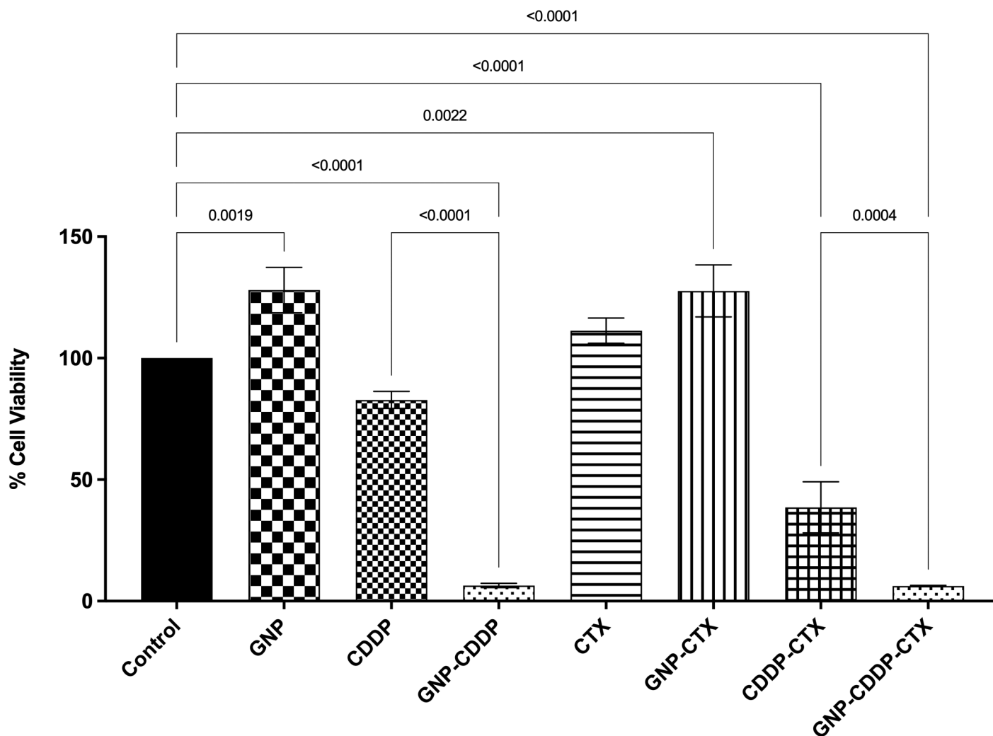
FIG. 6. The effects of nanodrug complex on cell viability in UPCI-SCC-131. Cells were incubated with 25 \mu\text{g}/\text{mL} GNPs, 2.5 \mu\text{g}/\text{mL} CDDP, and 25 \mu\text{g}/\text{mL} CTX for 48 hours. The percentage of cell viability was determined by using cell index values in GNP-treated UPCI-SCC-131 cells. Data are expressed as mean \pm SD ( n = 3 ). P \leq .05 . GNP: Gold nanoparticle, CDDP: Cisplatin, CTX: Cetuximab.
