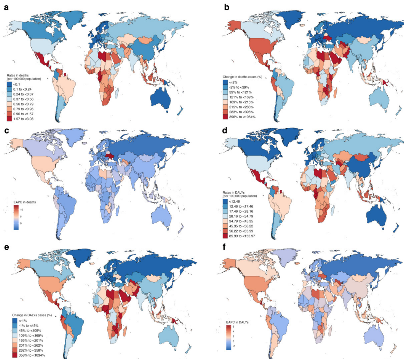
SUPPLEMENTARY FIG. 1. Global distribution of the burden of CKD attributable to high systolic blood pressure among young adults aged 25-49 years in 204 countries. (a) Death rates attributable to high SBP-related CKD by country in 2021. (b, c) Absolute change in the number of deaths and EAPC in death rates attributable to high SBP-related CKD from 1990 to 2021 by country. (d) DALY rates per 100,000 population attributable to high SBP-related CKD by country in 2021. (e, f) Absolute change in the number of DALYs and EAPC in DALY rates attributable to high SBP-related CKD from 1990 to 2021 by country. CKD, chronic kidney disease; DALY, disability-adjusted life year; EAPC, estimated annual percentage change.
